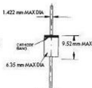
DO-201
