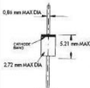
DO-41
