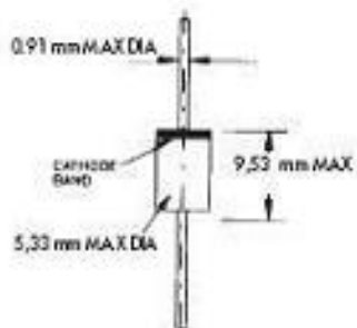
DO-27
